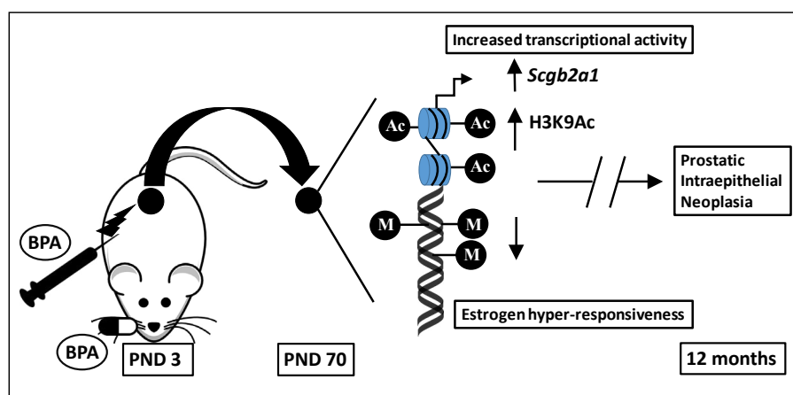
Figure 1. Early-life exposure to BPA results in increased enrichment of acetylated H3K9 (H3K9Ac representing active chromatin status) and hypomethylation of DNA for a CpG island upstream of the transcription start site of Scgb2a1 . M: Methyl; Ac: Acetyl; PND: postnatal days; BPA: Bisphenol A.
