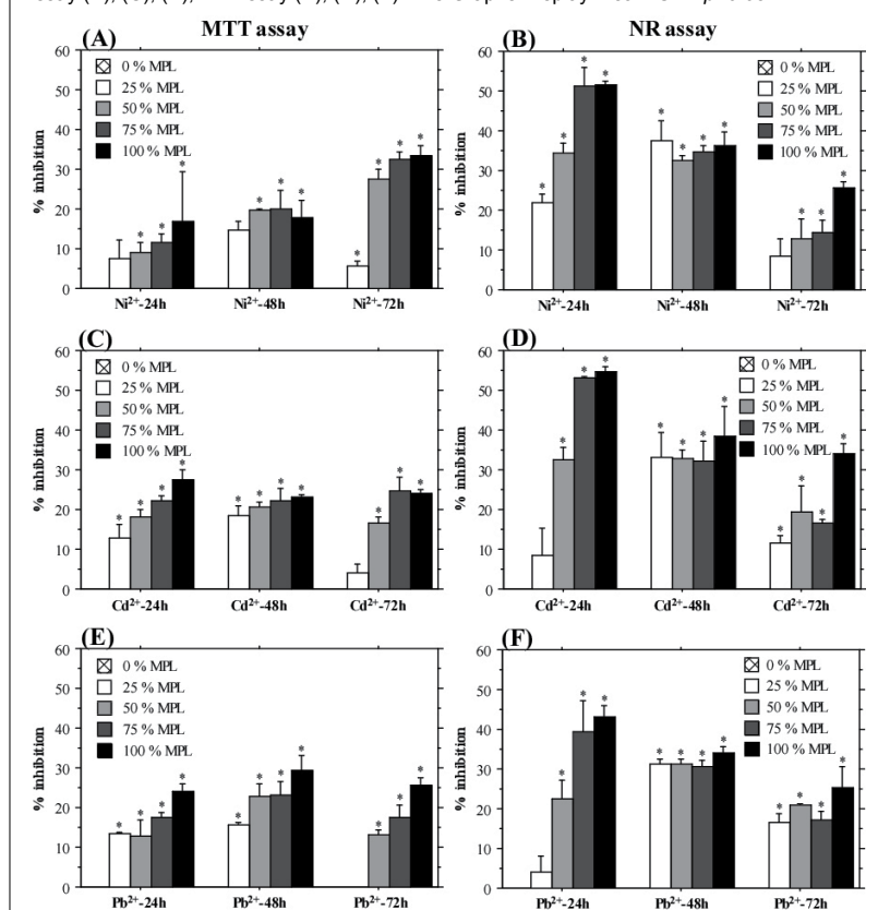
Figure 4: Inhibition of A549 Cells Growth after Treatment with Cadmium, Nickel and Lead. MTT Assay (A), (C), (E); NR Assay (B), (D), (F). The Graphs Display Mean±SE. *p<0.05.
