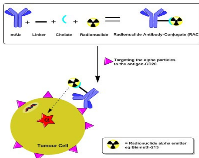
Figure 1: TAT targeting CD20 antigens on tumour cells
