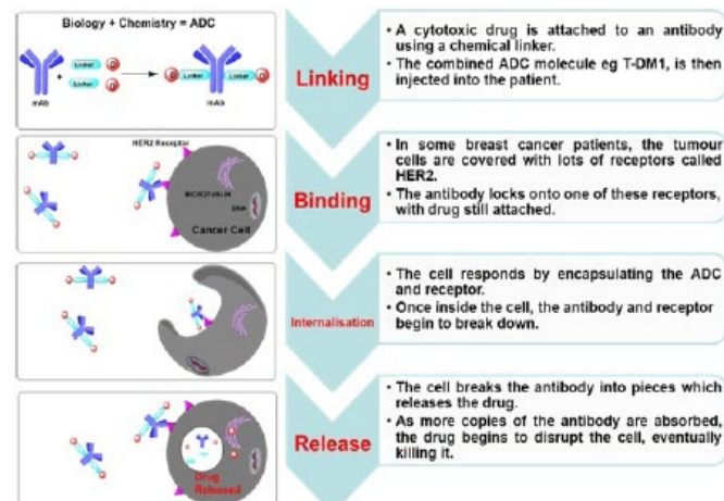
Figure 5: Mechanism of Action of ADCs
