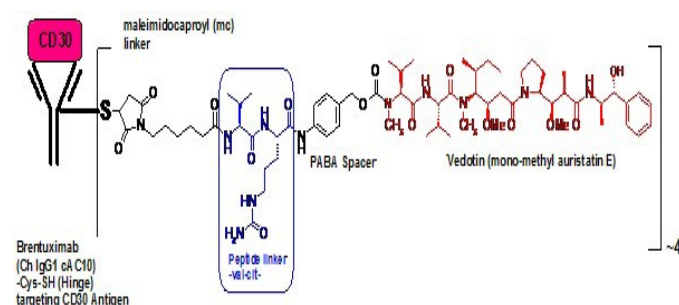
Figure 4: Structure of Adcetris ®
