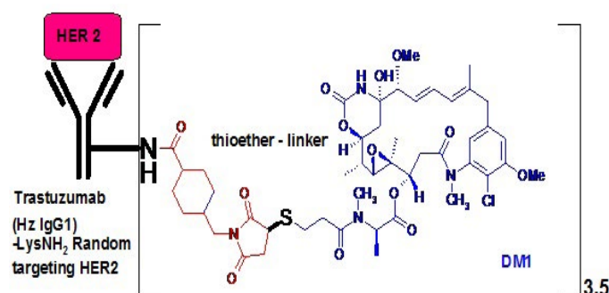
Figure 6: Structure of Kadcylla ®
