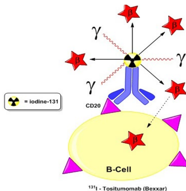
Figure 2: Bexxar® firing beta and gamma radiation to kill B-cells (Adaptation from Kitson et al. [51])
