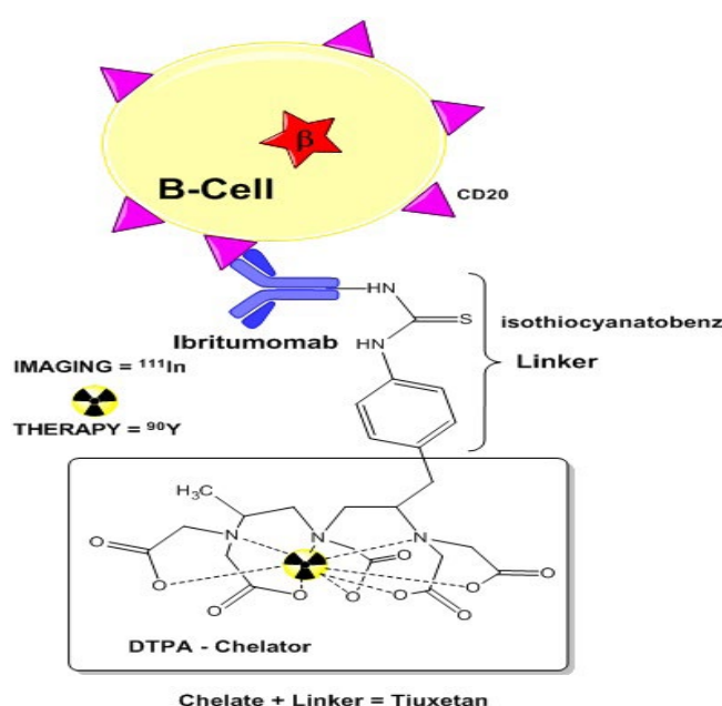
Figure 3: Zevalin® firing beta-particles at B-cells (Adaptation from Kitson et al. [51])
