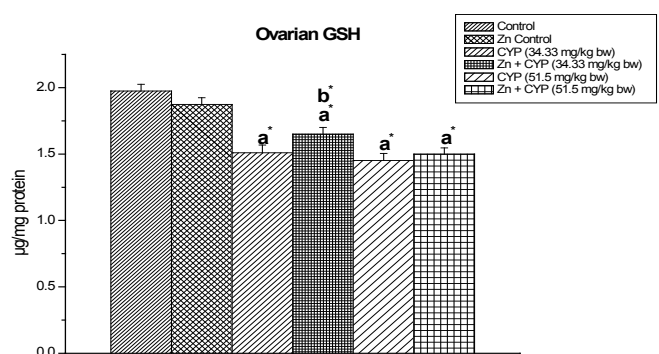
Figure 10: Effect of zinc on ovarian reduced glutathione (GSH) content in cypermethrin-exposed female prepubertal rats. Results are expressed as Mean \pm SEM. Analysis is done by ANOVA followed by multiple comparison two-tail t -tests. Superscript a Group I versus all other groups; superscript b Group III versus Group IV (*indicates p < 0.05 ).
