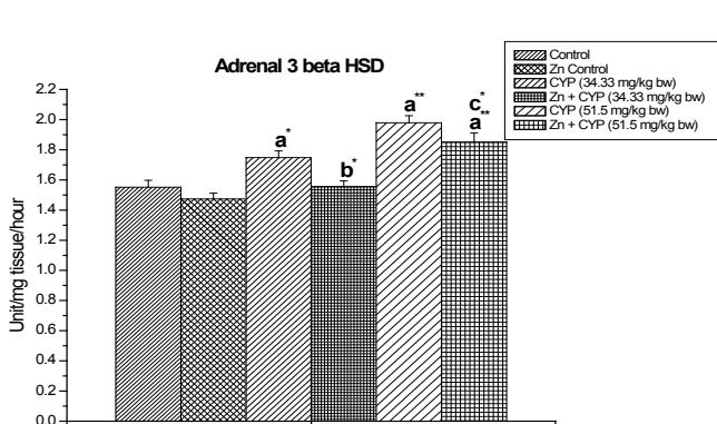
Figure 7: The effect of zinc on adrenal \Delta^5,3\beta -HSD in cypermethrin induced female prepubertal rats. Results are expressed as Mean \pm SEM. Analysis is done by ANOVA followed by multiple comparison two-tail t -tests. Superscript a Group I versus all other groups; superscript b Group III versus Group IV and superscript c Group V versus Group VI (*indicates p < 0.05 , ** indicates p < 0.01 ).
