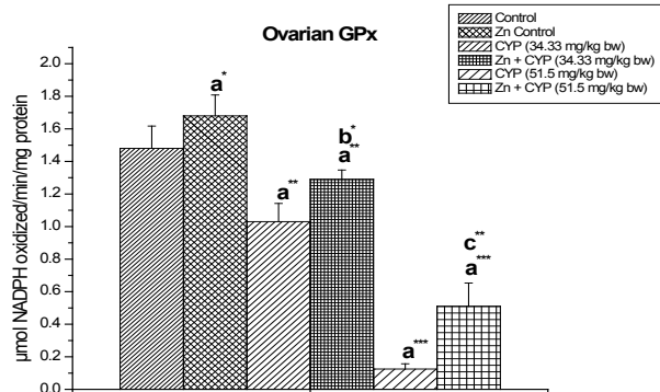
Figure 14: The effect of zinc on ovarian glutathione peroxidase (GPx) activity in cypermethrin-exposed female prepubertal rats. Results are expressed as Mean±SEM. Analysis is done by ANOVA followed by multiple comparison two-tail t -tests. Superscript a Group I versus all other groups; superscript b Group III versus Group IV and superscript c Group V versus Group VI (*indicates p<0.05 , **indicates p<0.01 and ***represents p<0.001 ).
