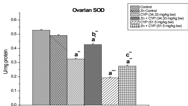
Figure 11: The effect of zinc on ovarian superoxide dismutase (SOD) activity in cypermethrin induced female prepubertal rats. Results are expressed as Mean±SEM. Analysis is done by ANOVA followed by multiple comparison two-tail t -tests. Superscript a Group I versus all other groups; superscript b Group III versus Group IV and superscript c Group V versus Group VI (*indicates p<0.05 , ** indicates p<0.01 and *** represents p<0.001 ).
