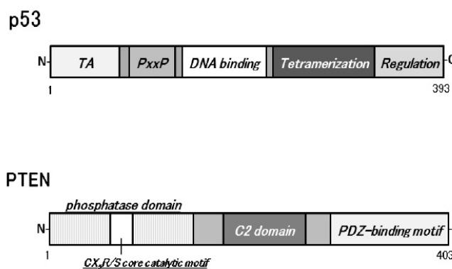
Figure 2: Schematic structures of p53 and PTEN proteins. The predicted consensual domain structures for each protein are depicted. The functionally important sites are shown. TA= trans-activation domain; PxxP= proline rich region; C2 domain= a protein structural domain involved in targeting proteins to cell membranes; PDZ= a common structural domain in signaling proteins (PSD95, Dlg, ZO-1, etc)
