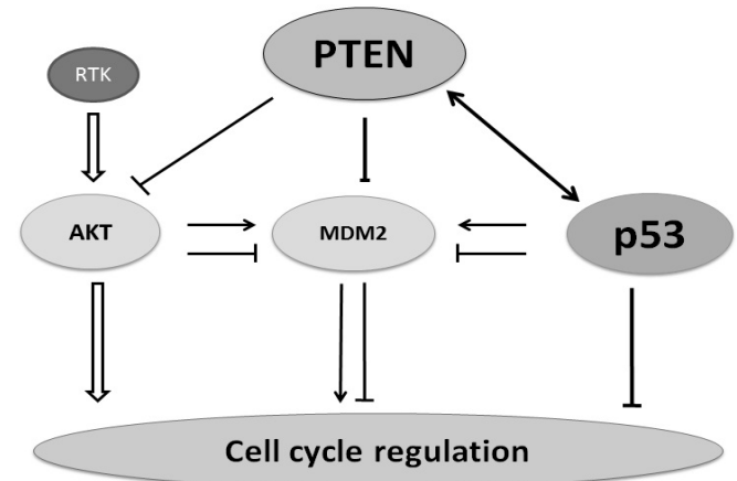
Figure 3: Suggestion of various regulatory loops involving the PTEN-p53-AKT-MDM2 network on cell cycle progression. Interactions are shown as arrows to mean activation, while hammerheads to mean inhibition. Note that some critical pathways have been omitted for clarity.
